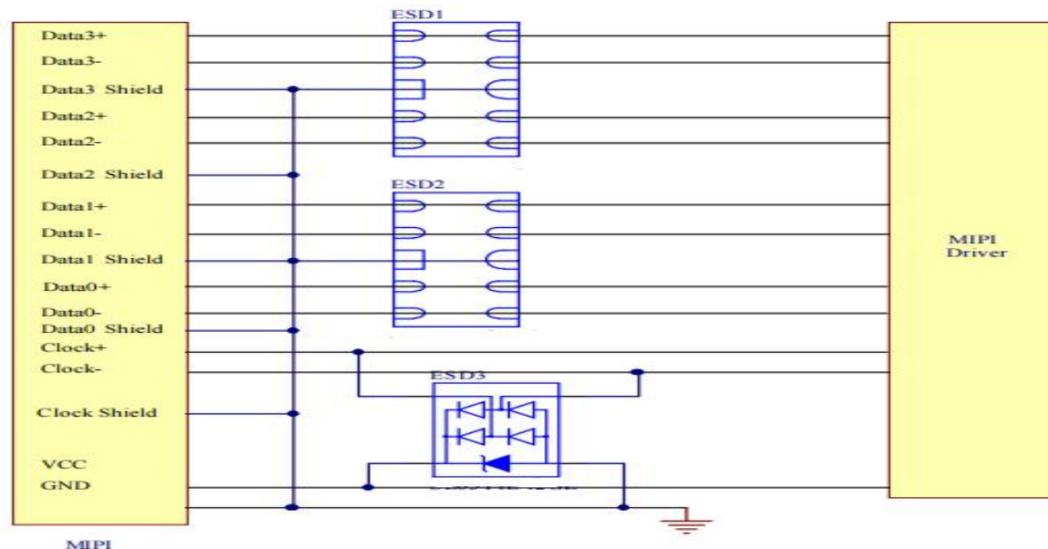
MIPI-DSI (LVDS)
