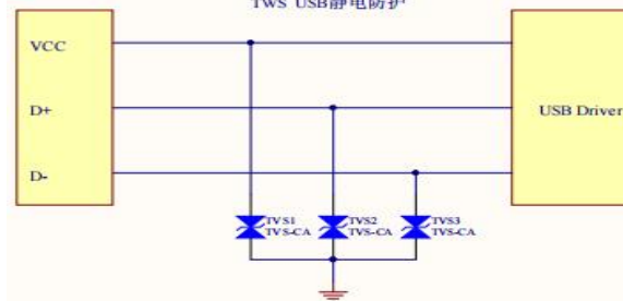
TWS USB静电防护
